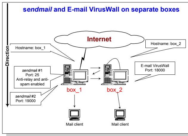
FIGURE 6-9. The illustration shows two Unix boxes configured to handle SMTP traffic. The arrows show the flow of traffic between boxes.
